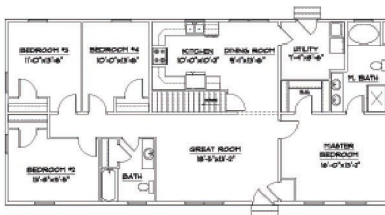
MAIN LEVEL PLAN
