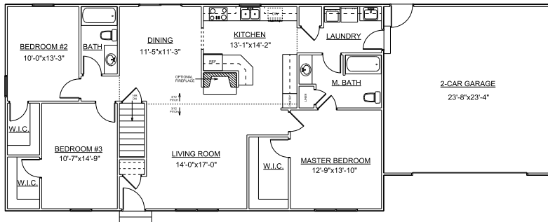
MAIN LEVEL PLAN
