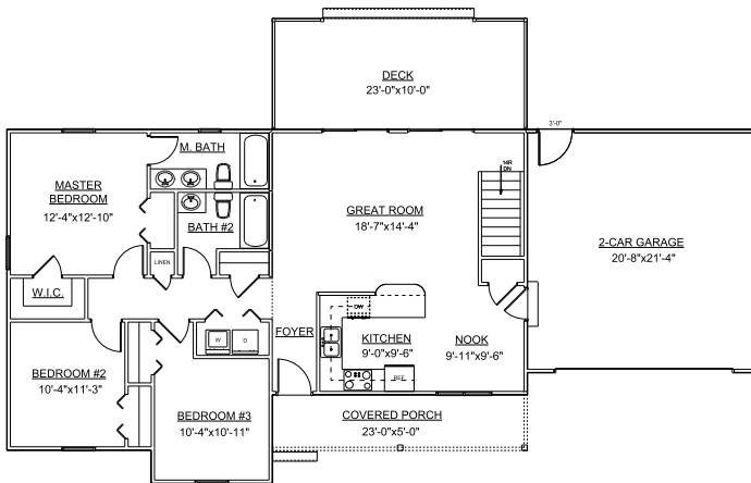
MAIN LEVEL PLAN
